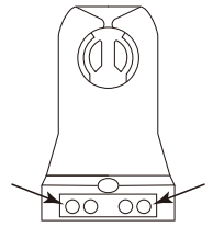
Non-shunted lampholder
