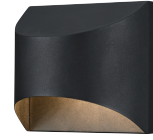
61228 Nardella LED Wall Fixture Textured Black Finish Height: 5.50" Width: 6.00" Extends: 4.25" Height from Center of Outlet Box: 2.76" Back Plate: H: 5.51" W: 5.91" Includes 10 Watt Integrated LED
